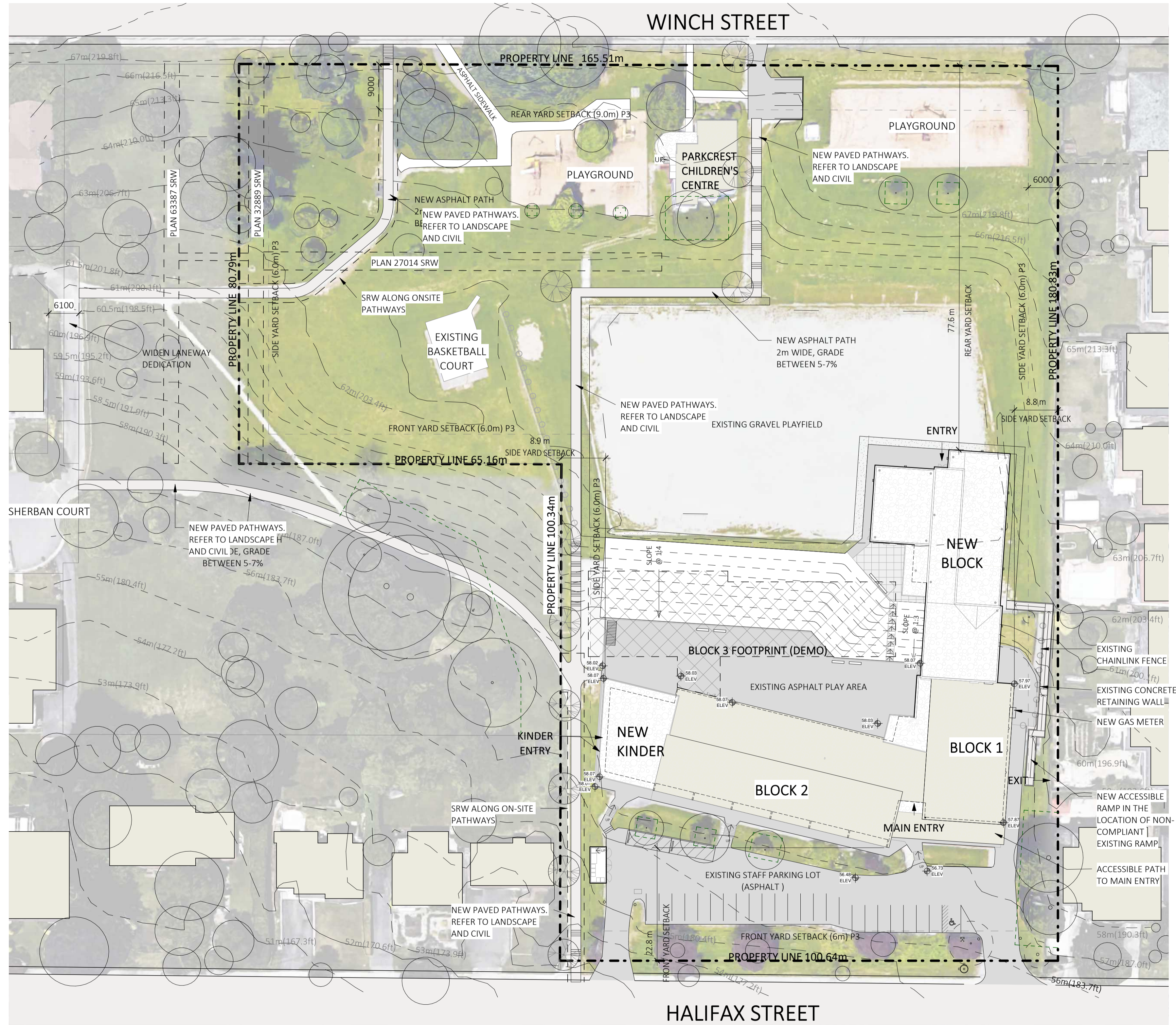
1 Proposed Site Plan 1 : 500
